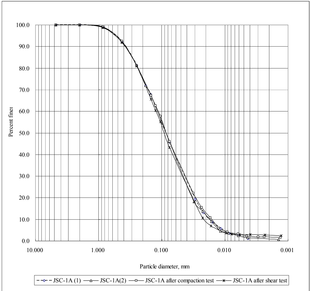
Figure 2. Particle size distribution of JSC-1A after compaction and shear test
