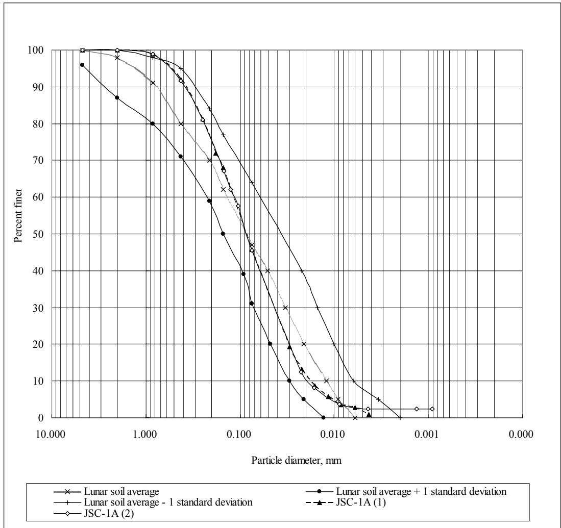
Figure 1. Particle size distribution of JSC-1A
