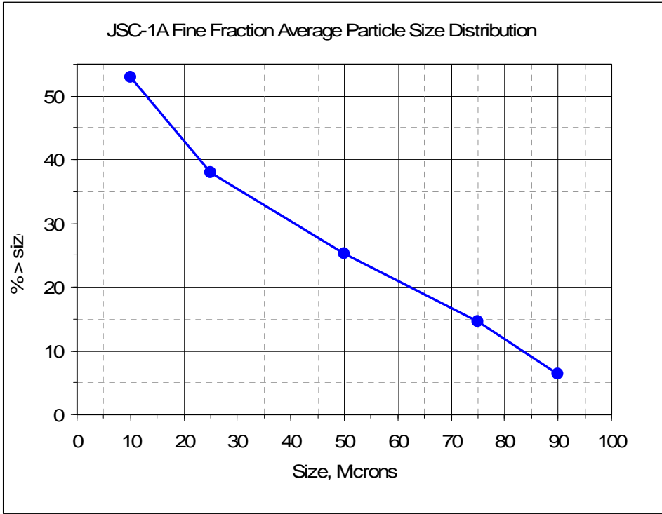
Figure 1. Average Particle Size Distribution for JSC-1A fine fraction.
